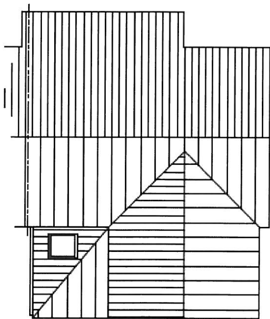
PROPOSED ROOF PLAN 1:100
